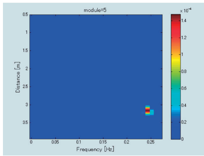
Fig. 13. Two dimensional maps of spectrum to distance from an antenna for a vibrating object located at three meters beneath the module No.5. Vibration frequency is 0.25Hz. Pulses are transmitted from an antenna in module No.5. Reflected waves are received by four antennas in module No.5.
